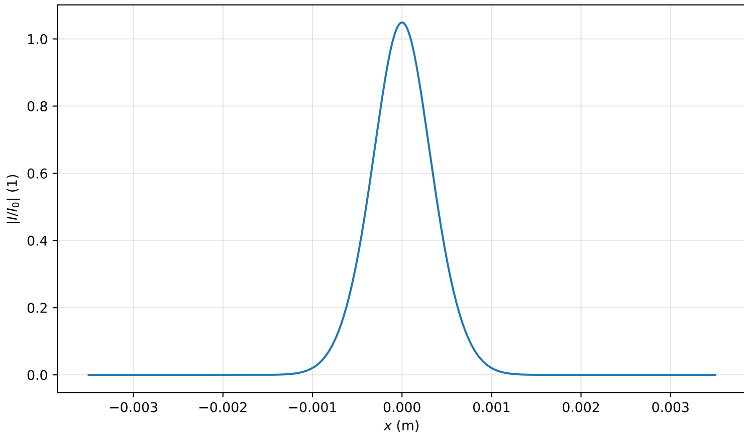
Intensity profile I(x, y = 0, z = 0.557m)/I_0 , P_{in}=0.5P_{cr} , artificial time
